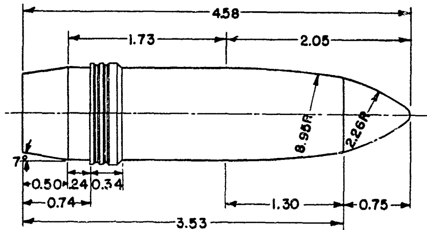
SHELL, HE, 90MM, M71 FUZE, CP, M78
