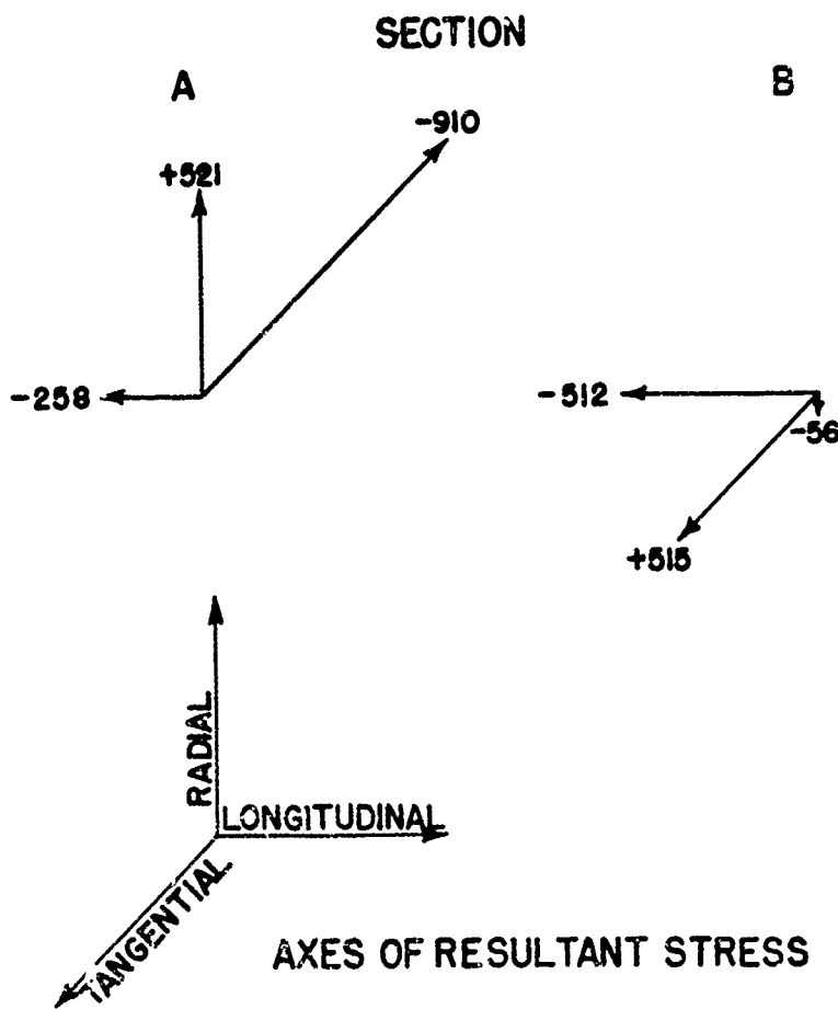
DIAGRAM OF RESULTANT STRESSES
