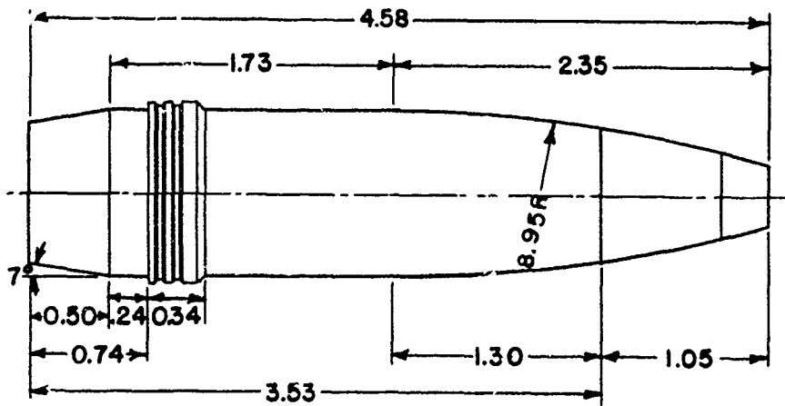
SHELL, HE, 90MM, M71 FUZE, MT, M43A5; PD, M48, M48AI OR M48A2; OR TSQ, M54
