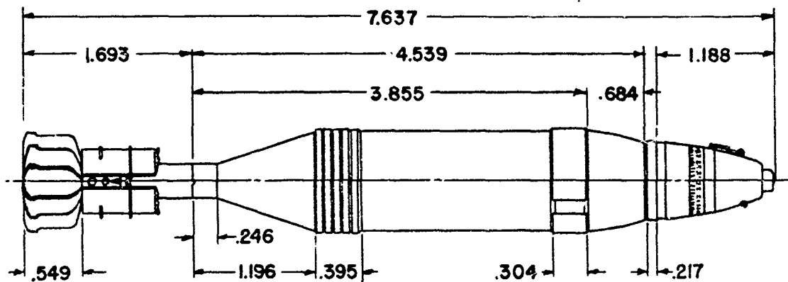
SHELL, SMOKE, 81-MM, M57 FUZE, T SQ., M77
